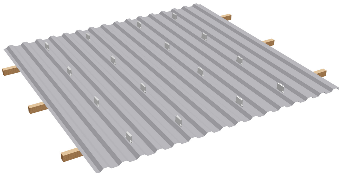
Completed installation of the rail layer.
