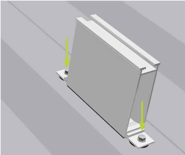
HS rail HK 125 XL 100
