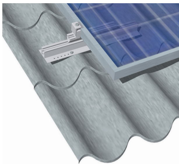
Differences in the levels of roof coverings featuring corrugated roof tiles are compensated
