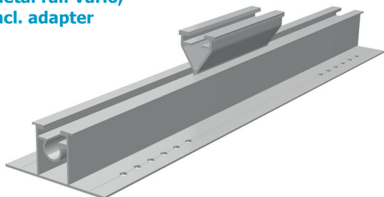
Differences in the levels of roof coverings featuring corrugated roof tiles are compensated
